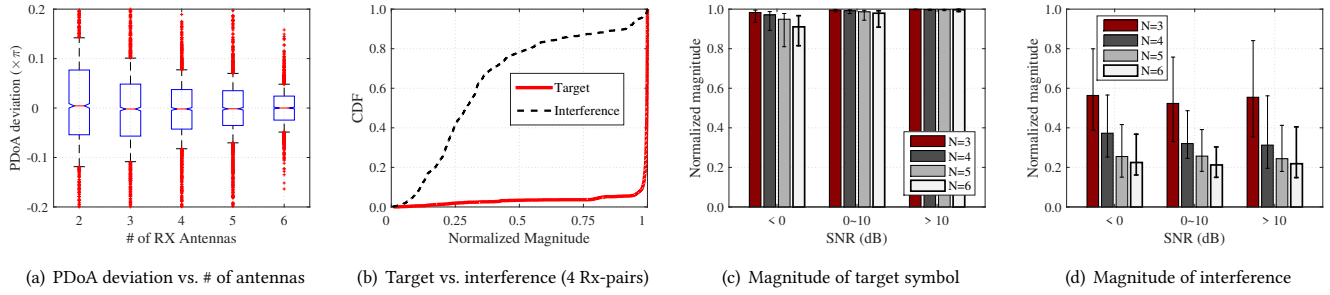
Figure 16: PDoA measurements with multiple antennas: (a) Impacts of multi-antenna on PDoA measurements (SNR<0dB), (b) Magnitudes of target symbols and interference when combining 4 Rx-pairs, (c,d) Impacts of antenna number (N) on magnitudes of target symbols and interference, respectively.
