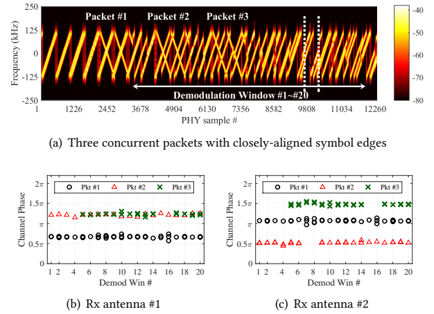
Figure 2: Reception diversities help decode more concurrent packets: air-channels of Packet #2 and Packet #3 have the same phase at antenna #1, all three packets have distinctive channel phases at antenna #2.
