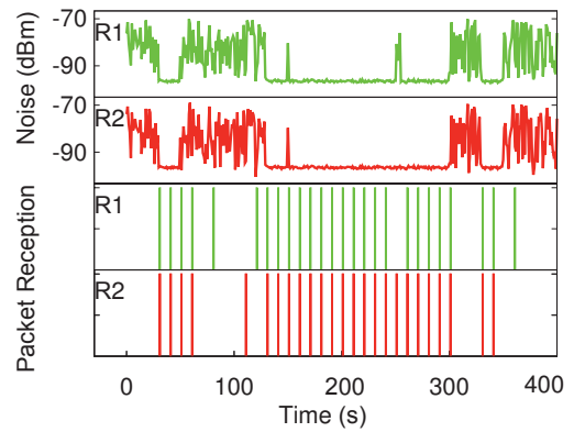
Fig. 1: Noise readings and packet receptions at receivers. Packet receptions are marked by vertical lines.
