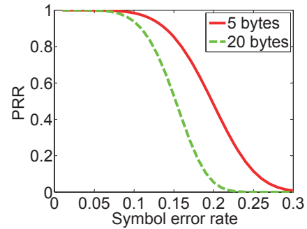
Fig. 3: The SER-PRR curves with different packet lengths.
