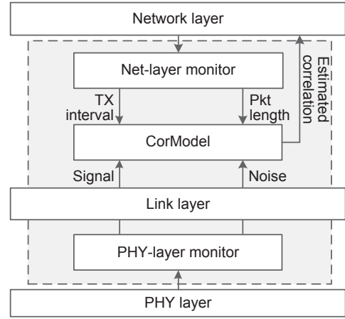
Fig. 6: Overview of CorModel estimation.
