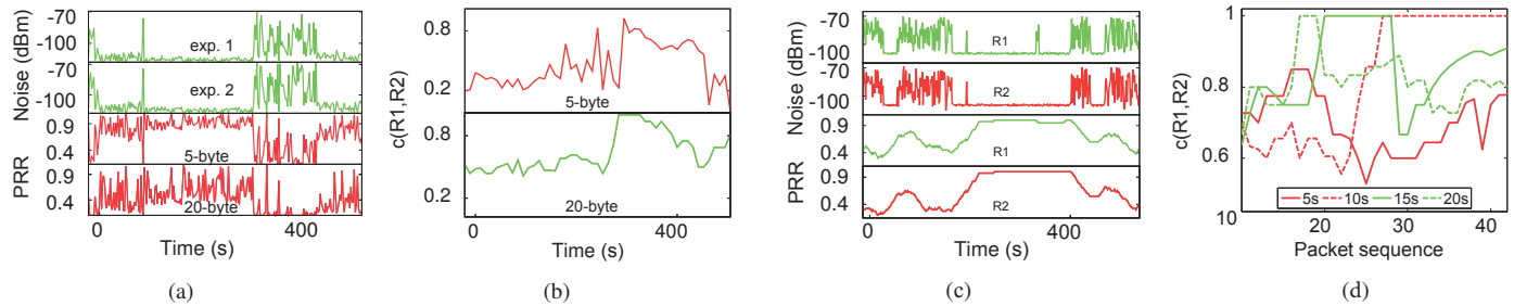
Fig. 4: Impact of network-layer parameters. (a) and (b) show the impact of packet length. (c) and (d) show the impact of data transmission interval.
