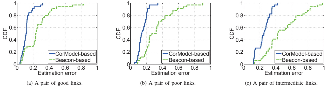
Fig. 7: Estimation accuracy comparison.
