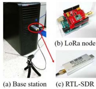
Fig. 10. Experiment devices.
