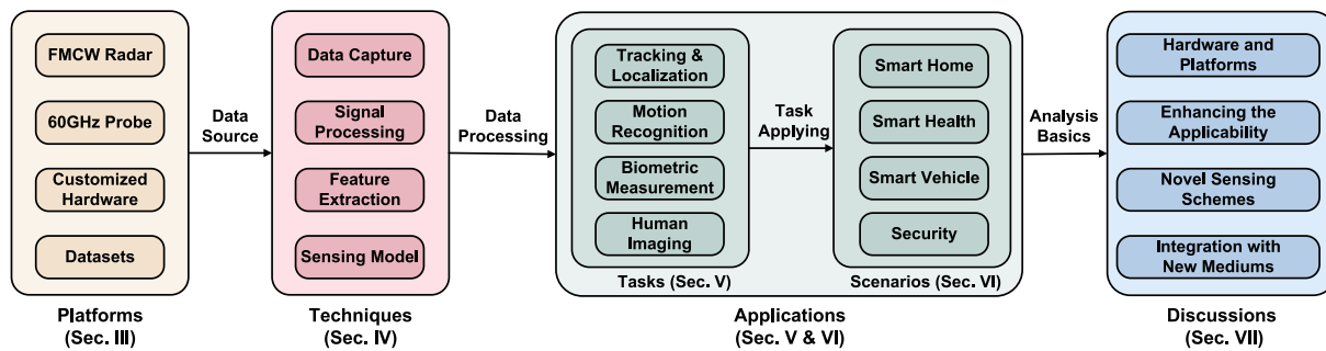
Fig. 1. Article organization.
