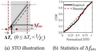
Fig. 7. Illustration of STO and empirical measurement results.
