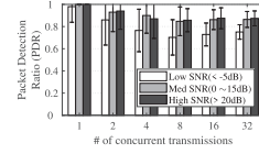
Fig. 23. Performance of concurrent packet detection.
