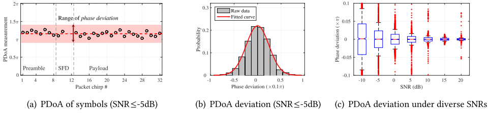
Fig. 16. PDoA measurements of a single packet: (a) PDoA measurements when \text{SNR} \leq -5\text{dB} , (b) PDoA deviation follows Gaussian distribution, (c) PDoA deviations under different SNRs.
