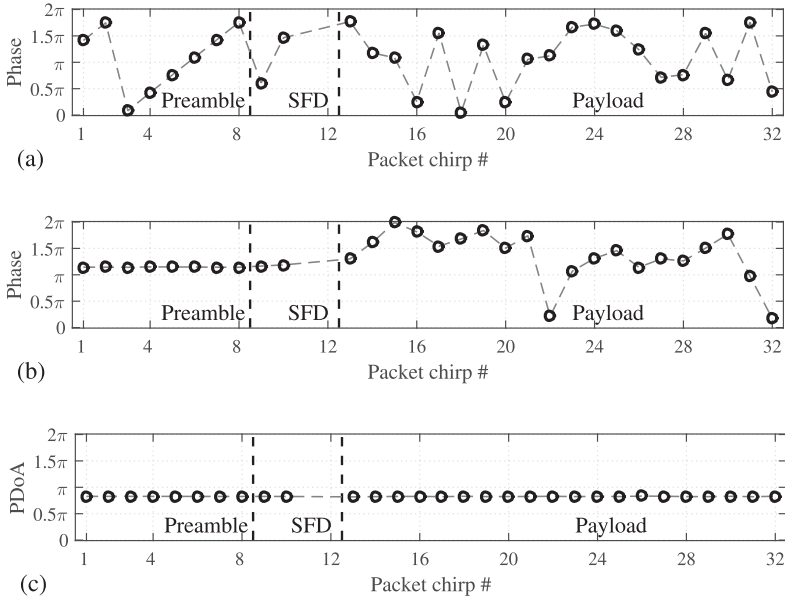
Fig. 9. Phase measurements: (a) from received raw signals; (b) after compensating for CFO and STO; (c) after calibrating for both frequency and phase.
