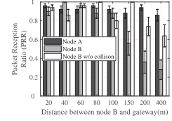
Fig. 21. Impact of near-far effects.
