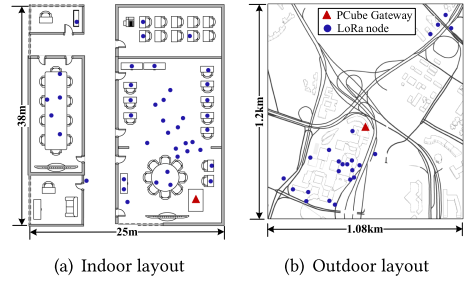
Fig. 15. Testbed settings of PCube.
