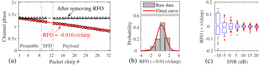
Fig. 10. Residual Frequency Offsets (RFOs) lead to drifts of measured channel phase (SF = 8, BW = 250 kHz): (a) RFO estimation and calibration, (b) RFO follows a Gaussian distribution (SNR ≥ 10 dB), (c) Impacts of SNR on RFO.
