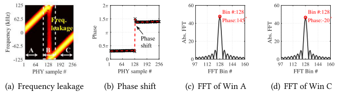
Fig. 8. Illustration of frequency leakage and impacts on phase measurements.
