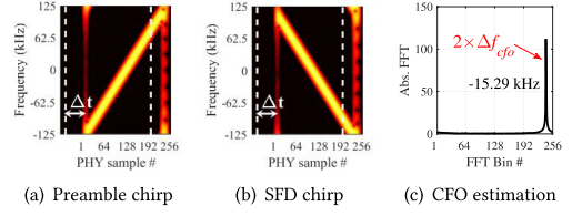
Fig. 6. Estimating CFO with preamble up-chirp and SFD down-chirp. The white dashed lines indicate the real chirp edges.
