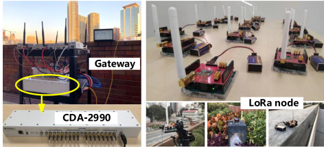
Fig. 14. PCube implementation.
