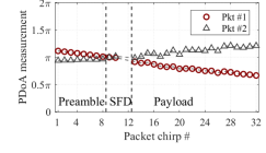
Fig. 24. PDOA of moving nodes.
