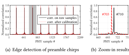
Fig. 5. Residual frequency offsets (i.e., CFO and STO) lead to incorrect detection of frame timing.
