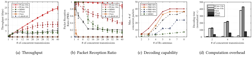
Fig. 19. Scalability evaluation: (a, b) Throughput and Packet Reception Ratio as the number of concurrent transmissions increases; (c) Decoding capability of PCube and MIMO; and (d) Comparison of computation overhead.
