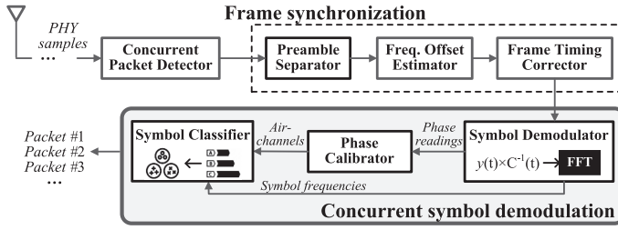
Fig. 13. Workflow of phase-based parallel decoding.
