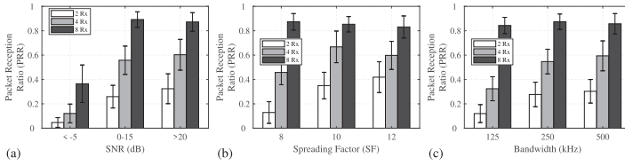
Fig. 20. Impacts of (a) SNR (b) spreading factor and (c) bandwidth on PCube when decoding 20 concurrent packets.
