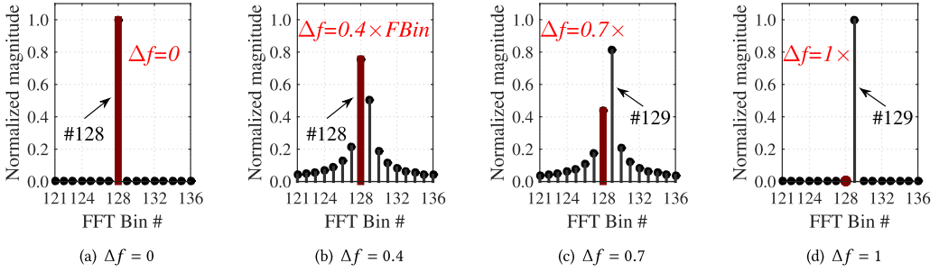
Fig. 4. FFT representation of fractional frequencies ( \Delta f ). F\text{Bin} denotes the frequency resolution of FFT.
