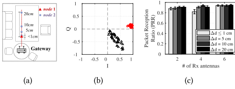
Fig. 22. Impact of proximity of node locations: (a) Experiment settings; (b) PDOA measurements from collided packets of two nodes when \Delta d \leq 1\text{ cm} ; and (c) Packet reception performance.
