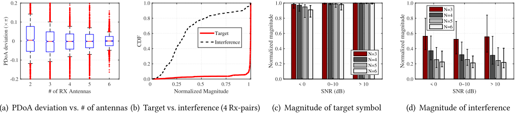
Fig. 18. PDoA measurements with multiple antennas: (a) Impacts of multi-antenna on PDoA measurements (SNR < 0dB), (b) Magnitudes of target symbols and interference when combining four Rx-pairs, (c, d) Impacts of antenna number ( N ) on magnitudes of target symbols and interference, respectively.
