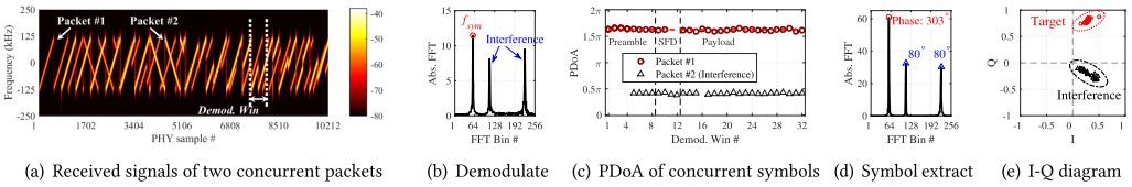
Fig. 11. Illustration of extracting PDoA for concurrent symbols and PDoA-based packet decoding.
